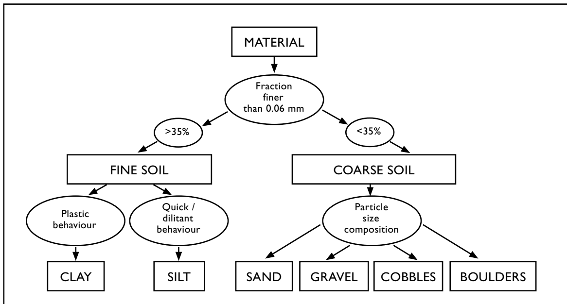
Figure 2.1 Soil Classification
